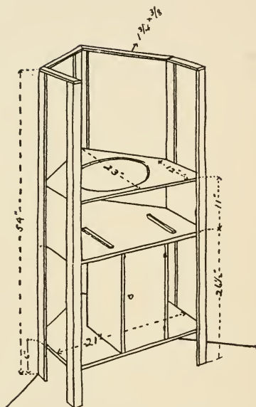
CORNER WASHSTAND
